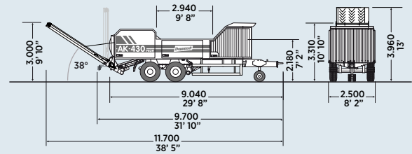
Transport dimensions L/W/H: 9.700/2.500/3.960
